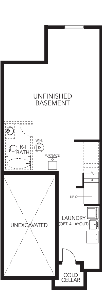
BASEMENT PLAN
