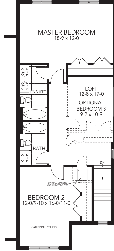
SECOND FLOOR PLAN OPT. 1
