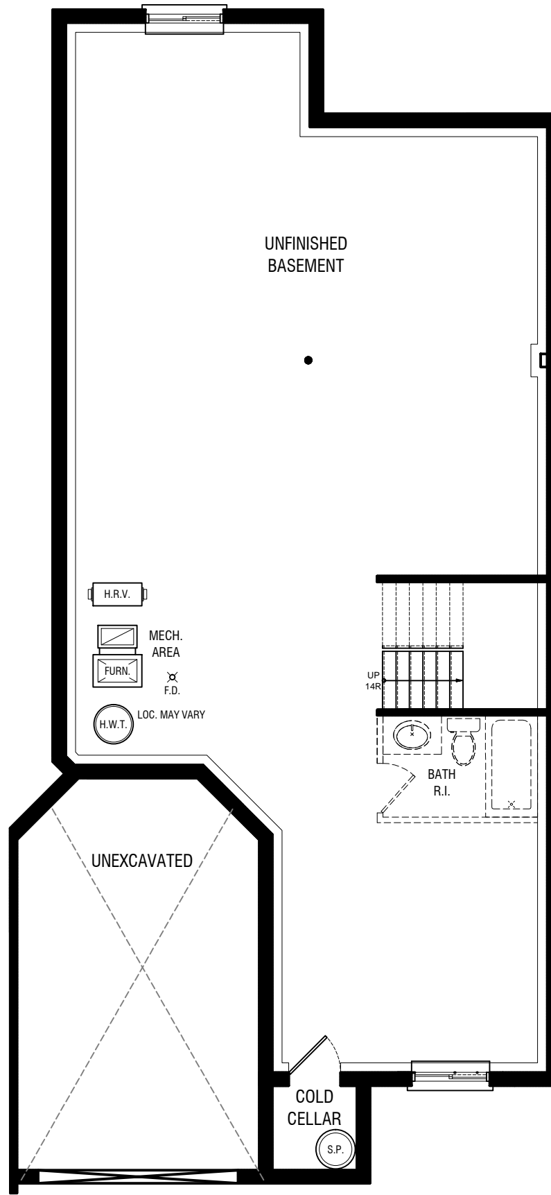
BASEMENT PLAN
