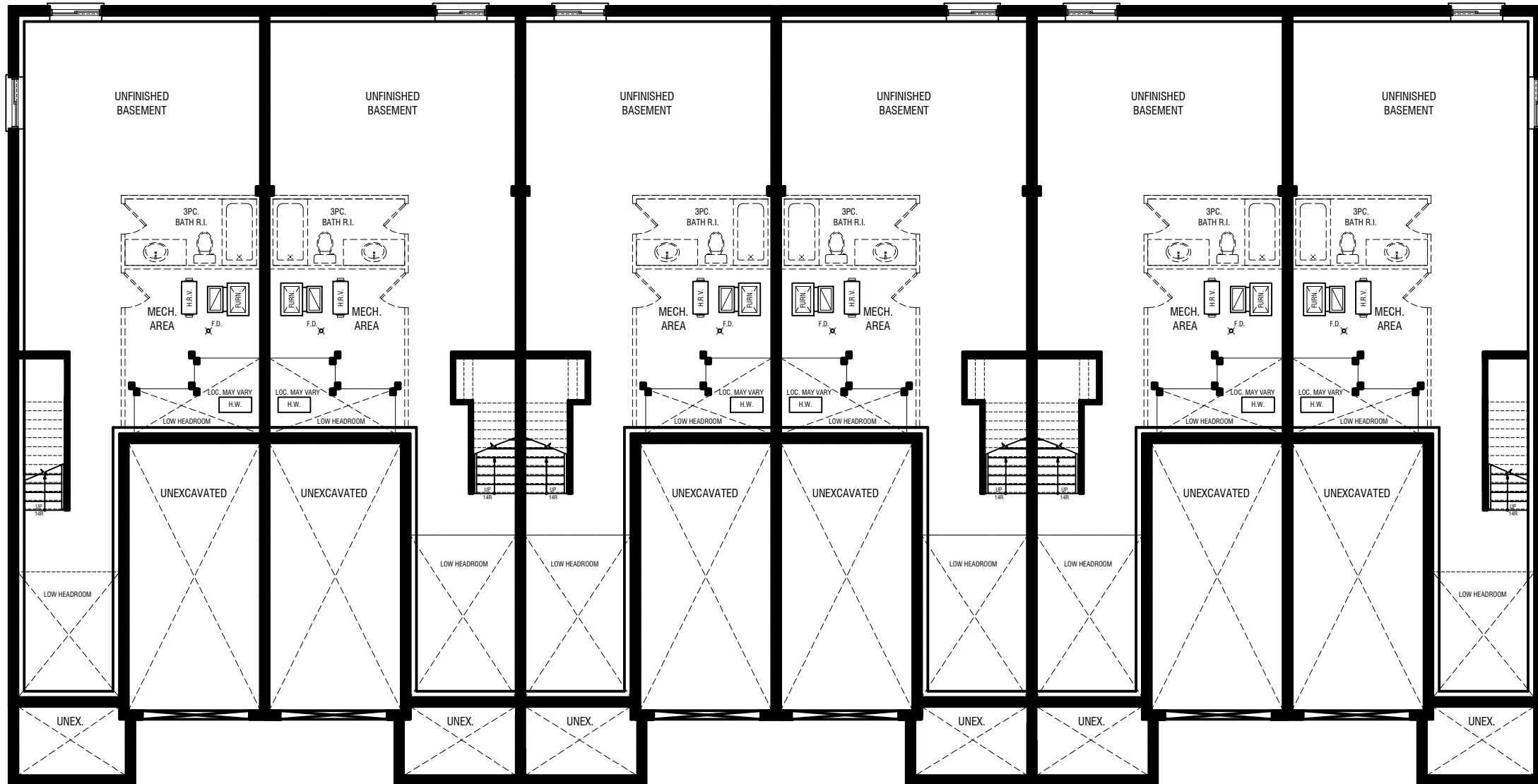
BASEMENT PLAN
